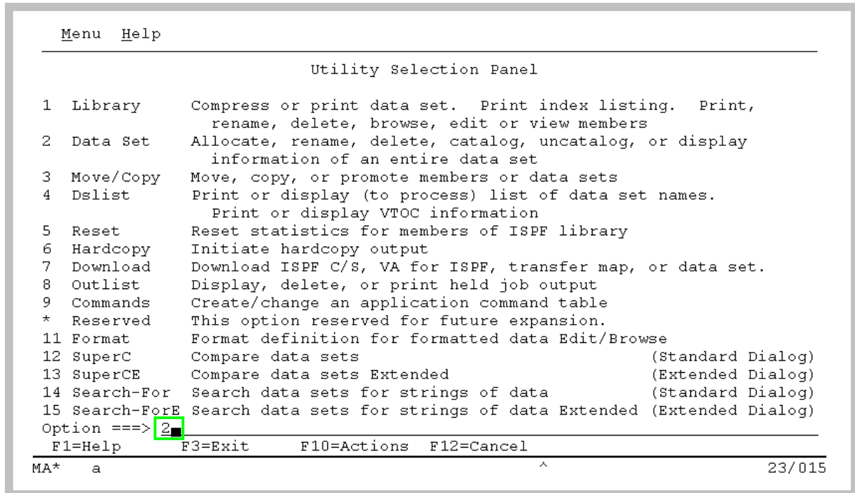
Abbildung 10: "Utility Selection Panel"-Bildschirm
